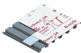
BlockShield SA Plus Head Lap over Metal Deck
