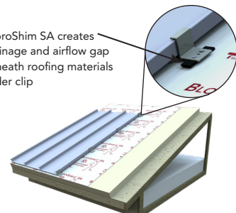
Vented Attic
